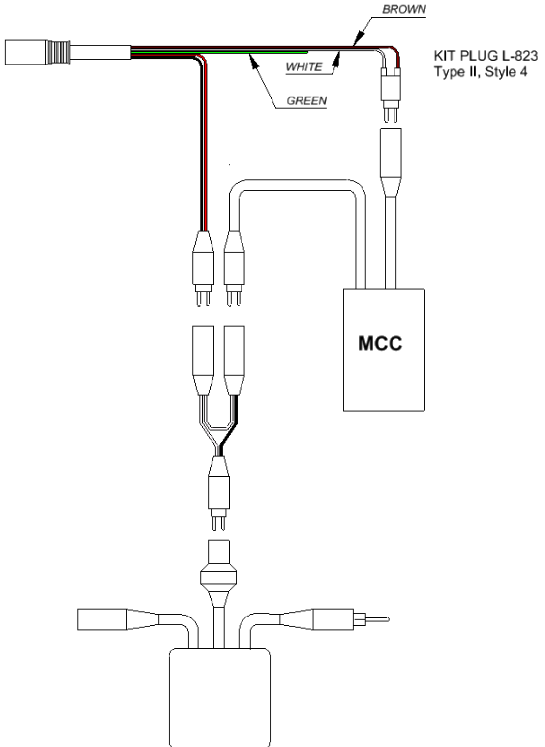
Figure 17 – Wiring diagram for connection of monitored LETG to transformer.
