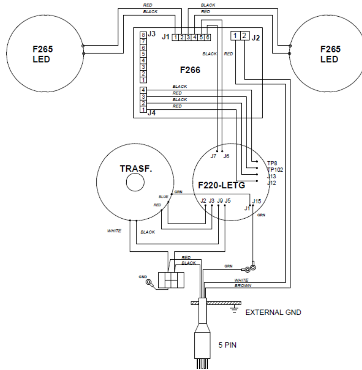
Figure 10– Monitored series circuit power supply
