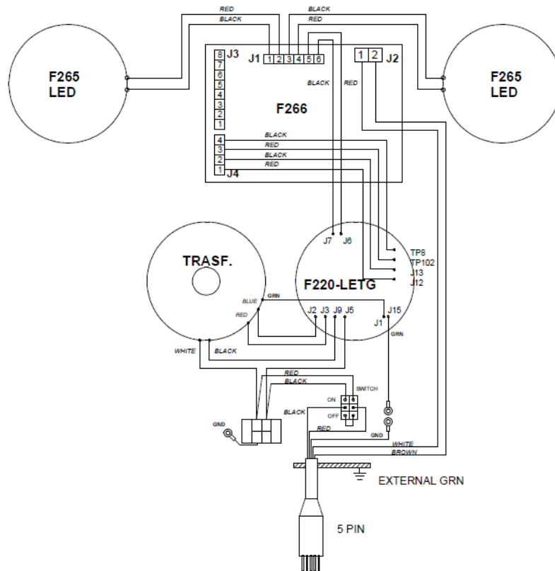
Figure 11– Monitored series circuit power supply with switch
