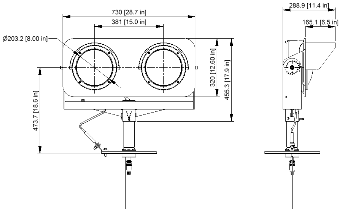
Figure 1 - Overall dimensions
